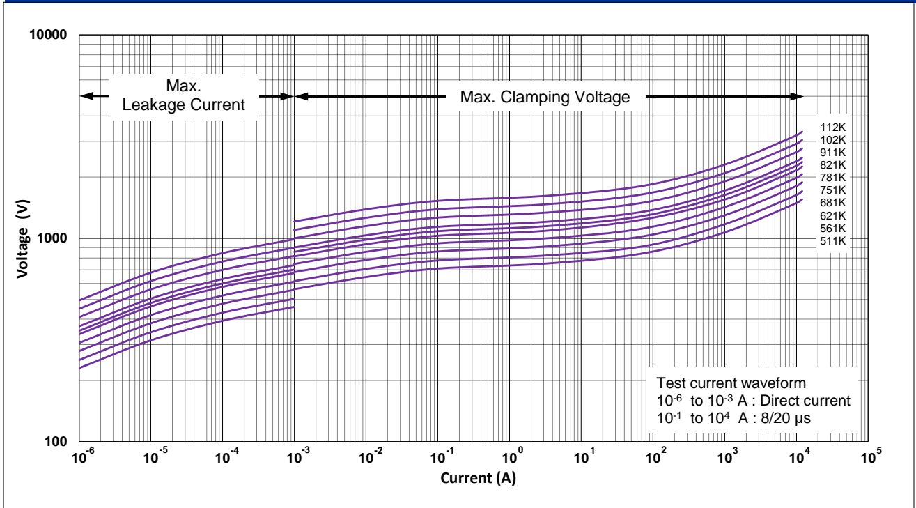
CNR-18P511K to 18P112K V-I Curves
