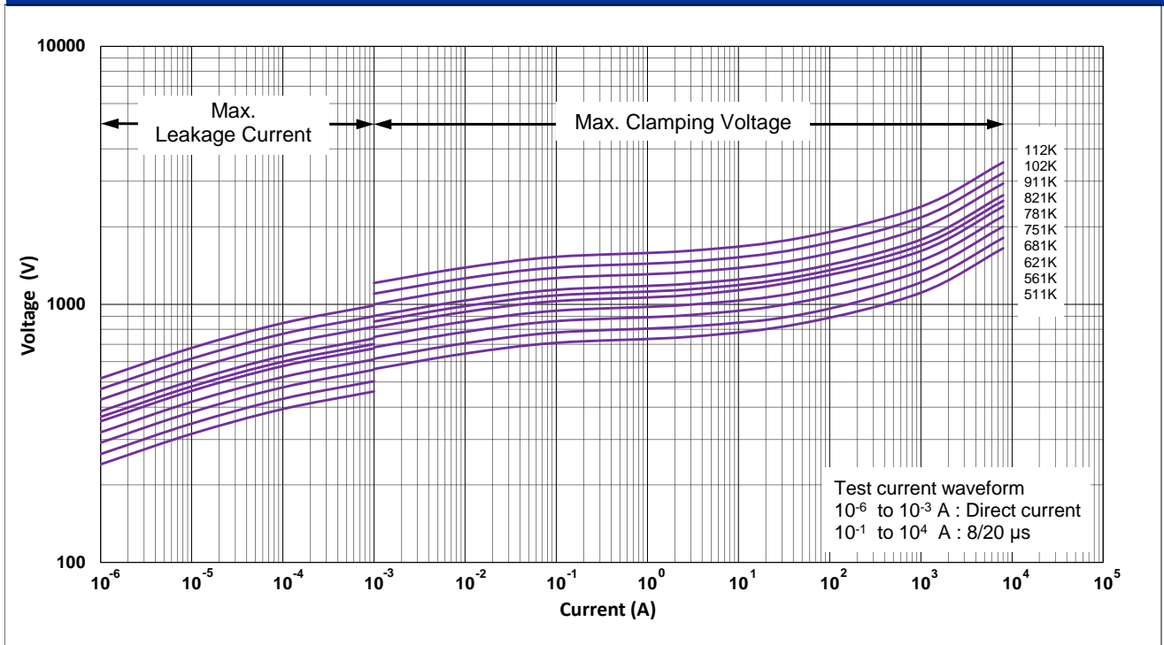
CNR- 14P511K to 14P112K V-I Curves
