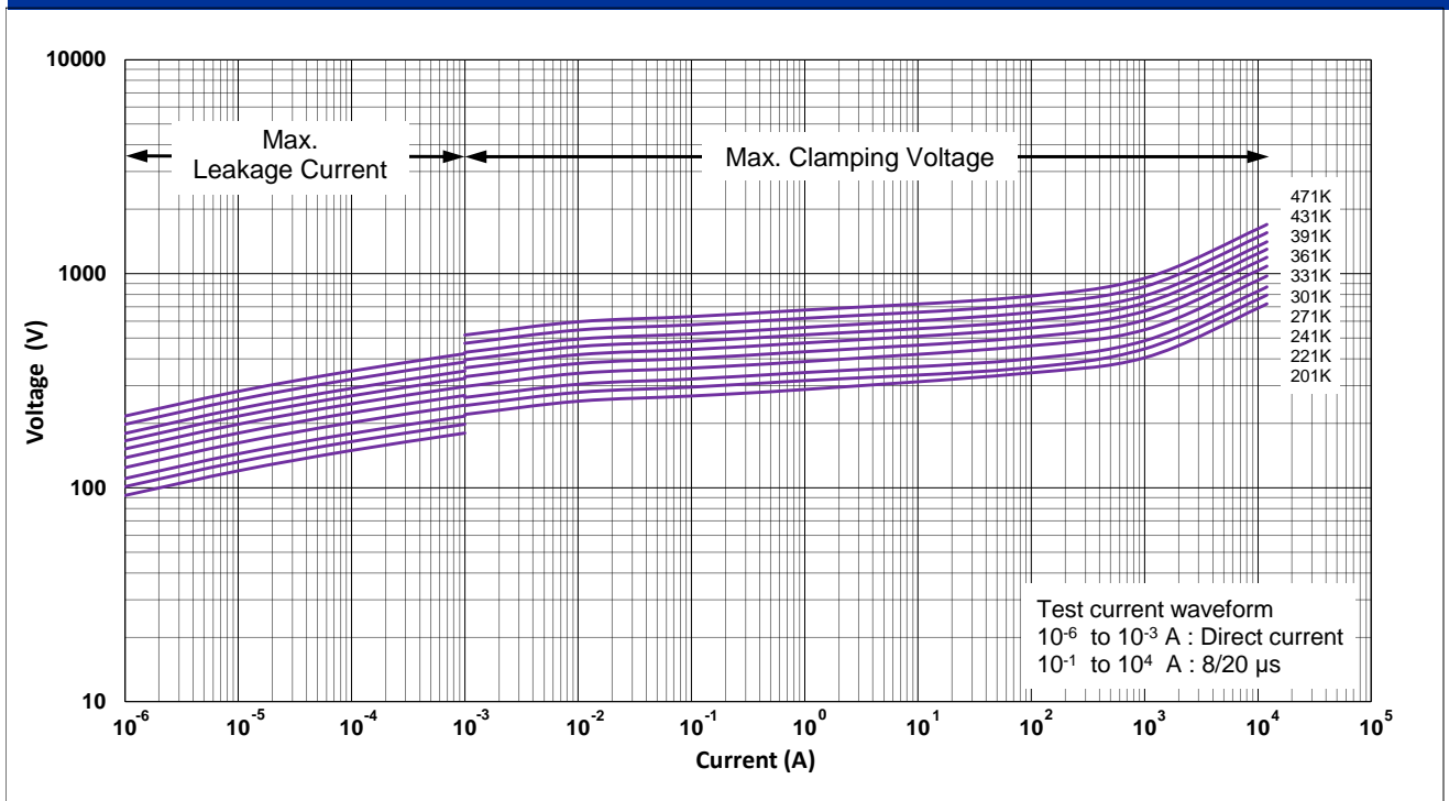
CNR-18P201K to 18P471K V-I Curves
