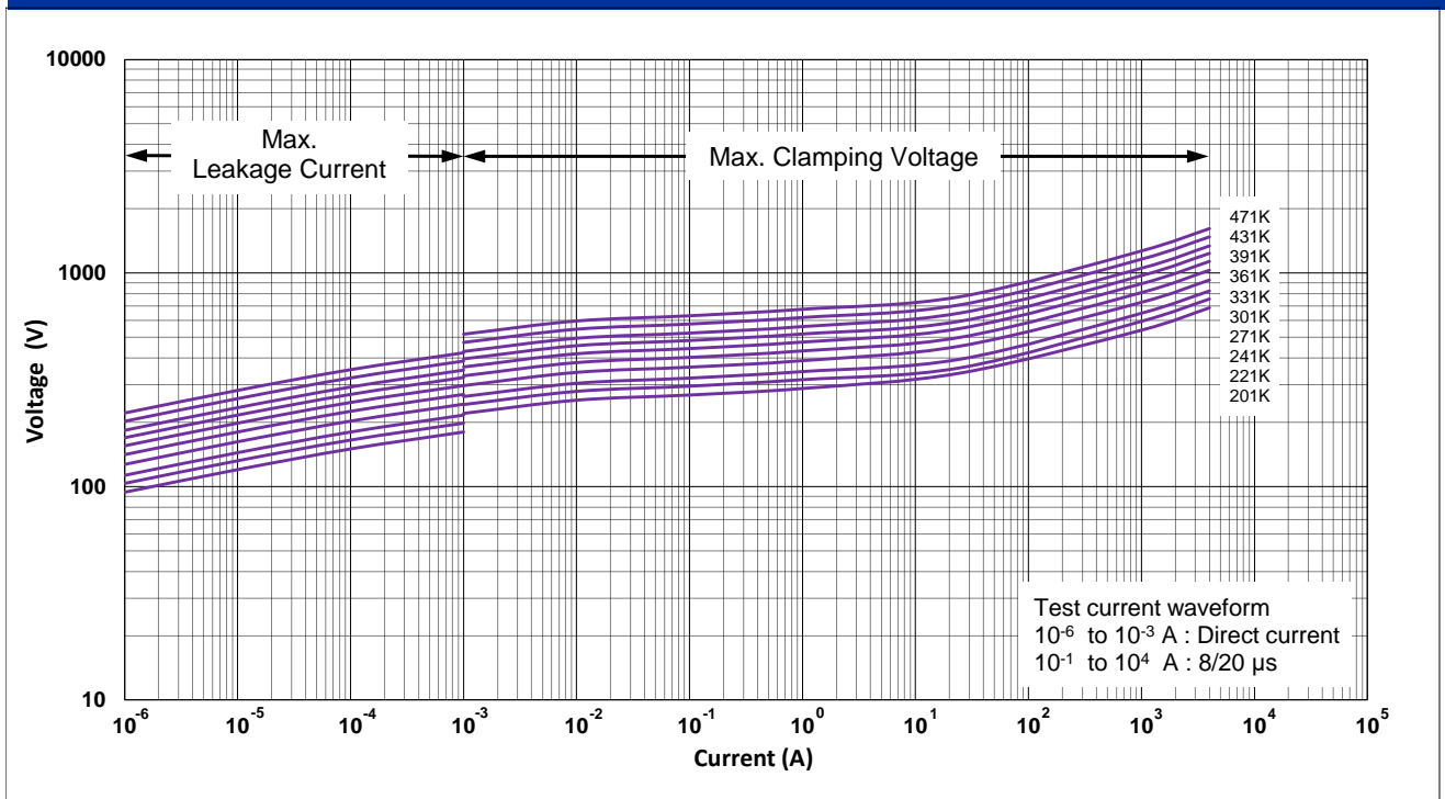
CNR-10P201K to 10P471K V-I Curves
