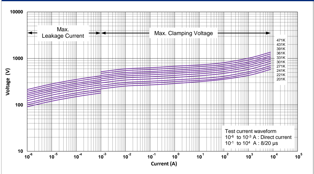
CNR-14P201K to 14P471K V-I Curves
