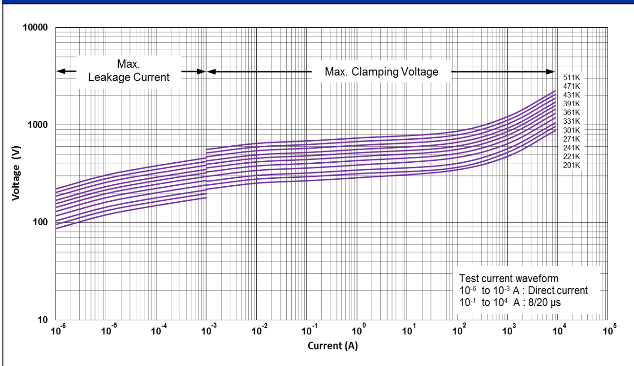
CNR-18V201K to CNR-18V511K V-I Curves
