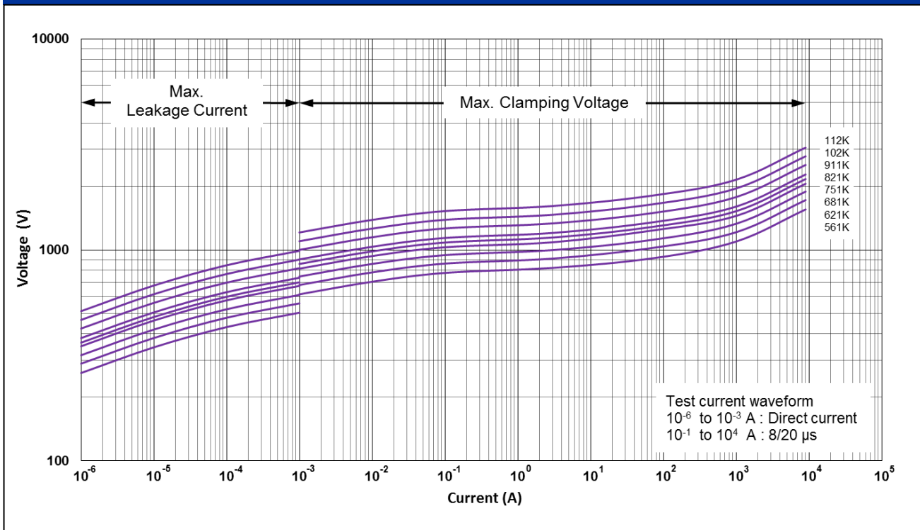
CNR-18V561K to CNR-18V112K V-I Curves
