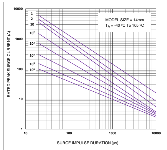
CNR-14V201K to CNR-14V112K
