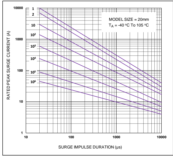
CNR-20V201K to CNR-20V112K
