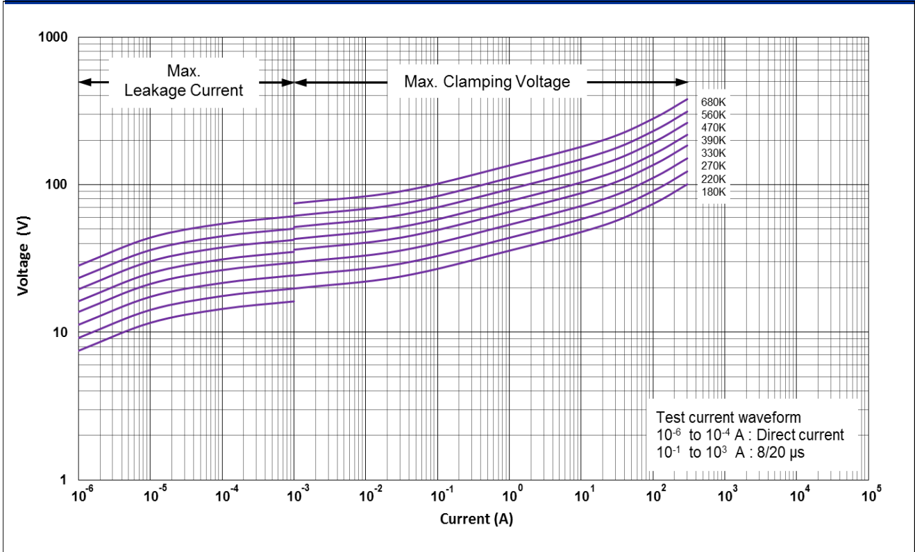
CNR-05N180K to CNR-05N680K V-I Curves
