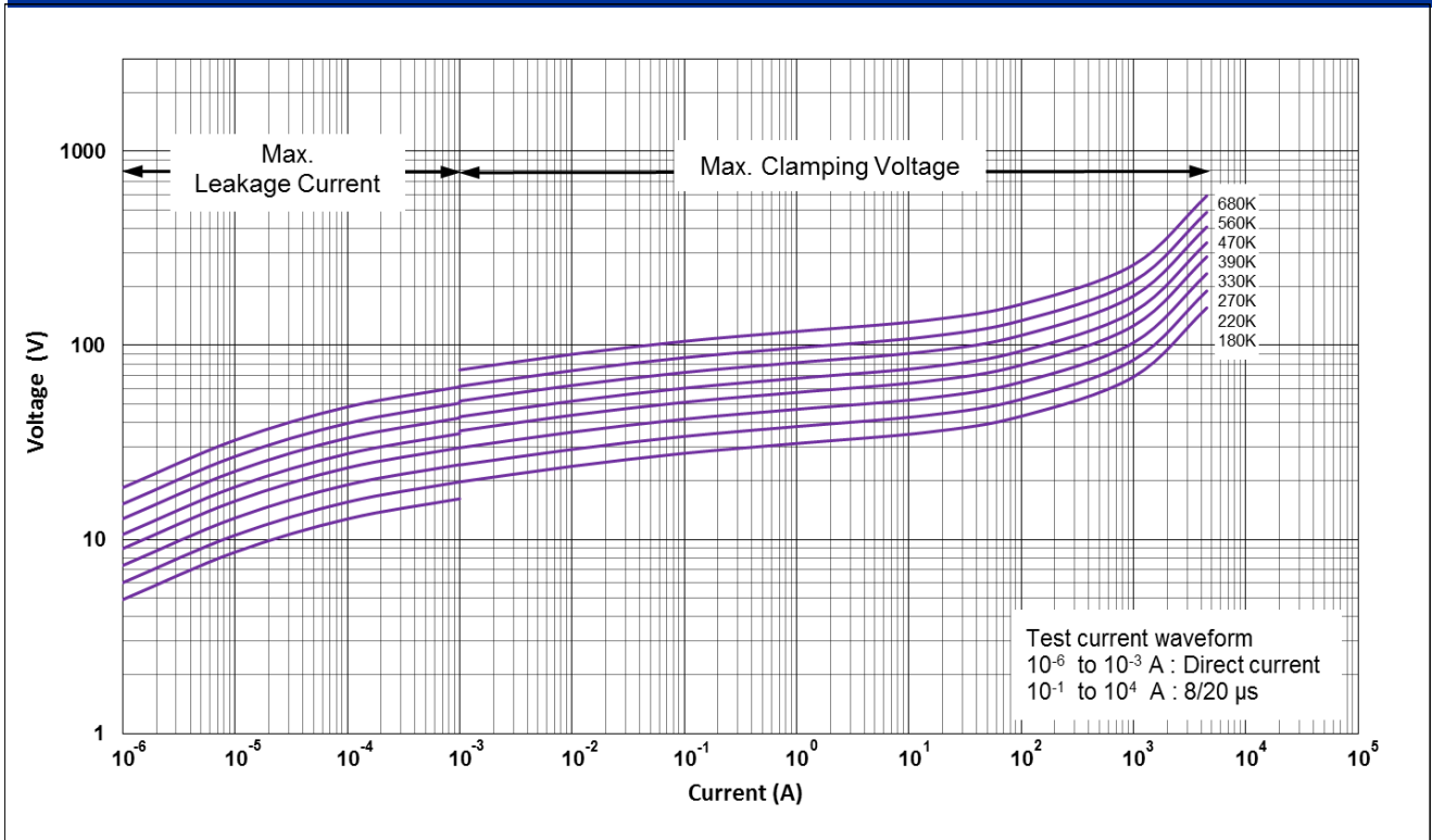
CNR-18N180K to CNR-18N680K V-I Curves
