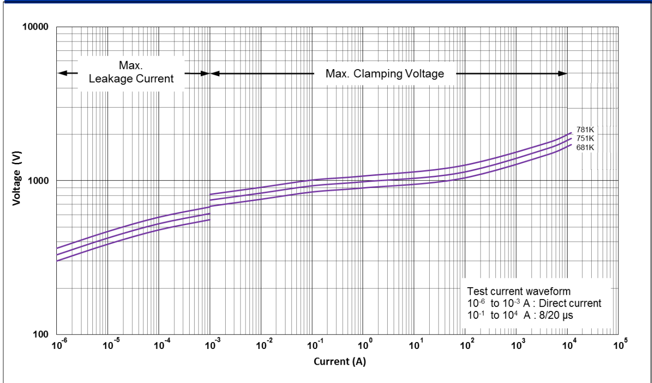
CNR-18N621K to CNR-18N751K V-I Curves
