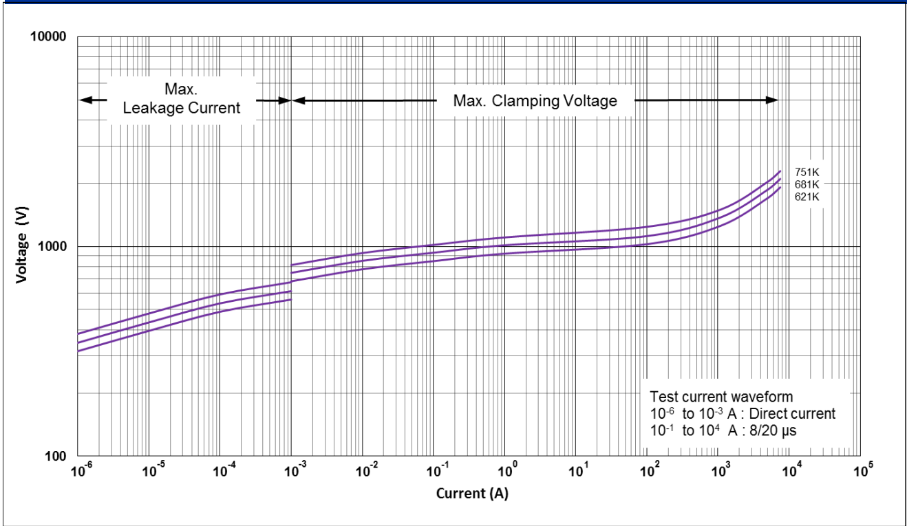
CNR-18N621K to CNR-18N751K V-I Curves
