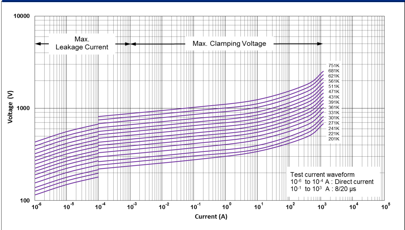
CNR-05N201K to CNR-05N751K V-I Curves
