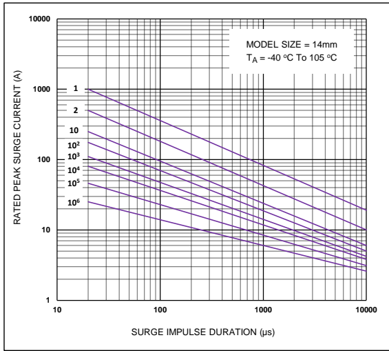
CNR-14D180K to CNR-14D680K
